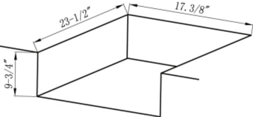
CUT OUT
